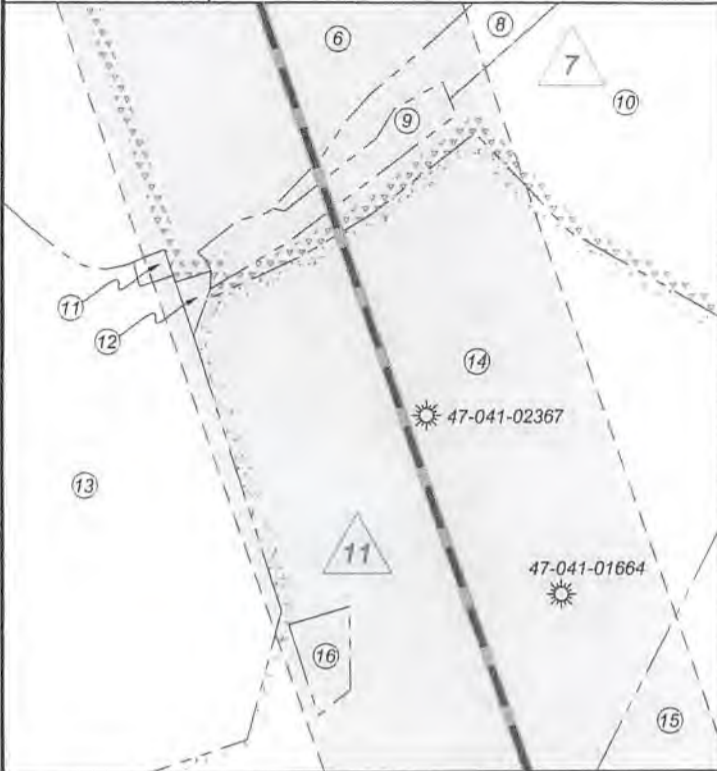
Detail 2 (1"=500')
