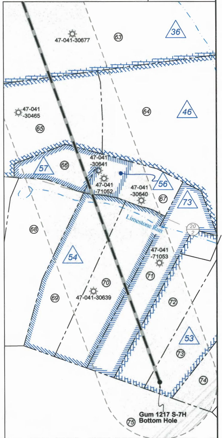
Detail 3 (Scale 1"=500')
