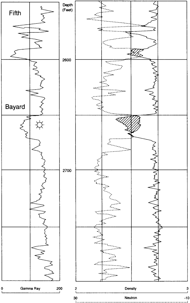
Figure Dvs-25. Type log of the Bayard sandstone (V-2), north-central West Virginia. The base of the Fifth sandstone is at 2,600 feet.
