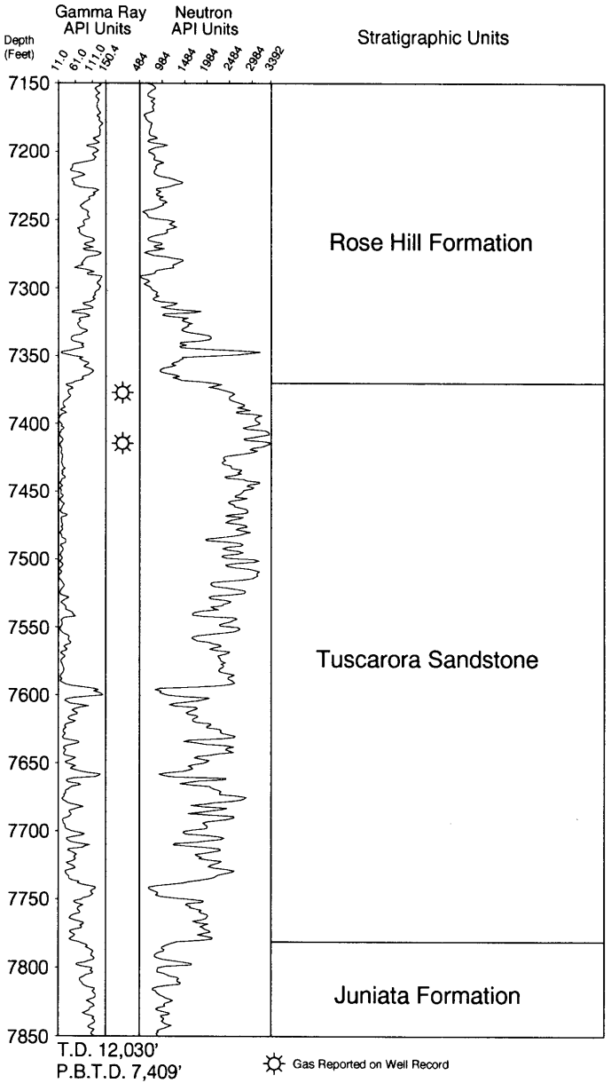
Figure Sts-16. Gamma-ray-laterolog-neutron log from Columbian Carbon Company No. N-1 (GW-1374) United States of America (Preston 99) showing the Tuscarora Sandstone in Leadmine field, Preston County, West Virginia.
