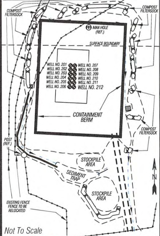
Detail Sketch for Proposed Well No. 212
