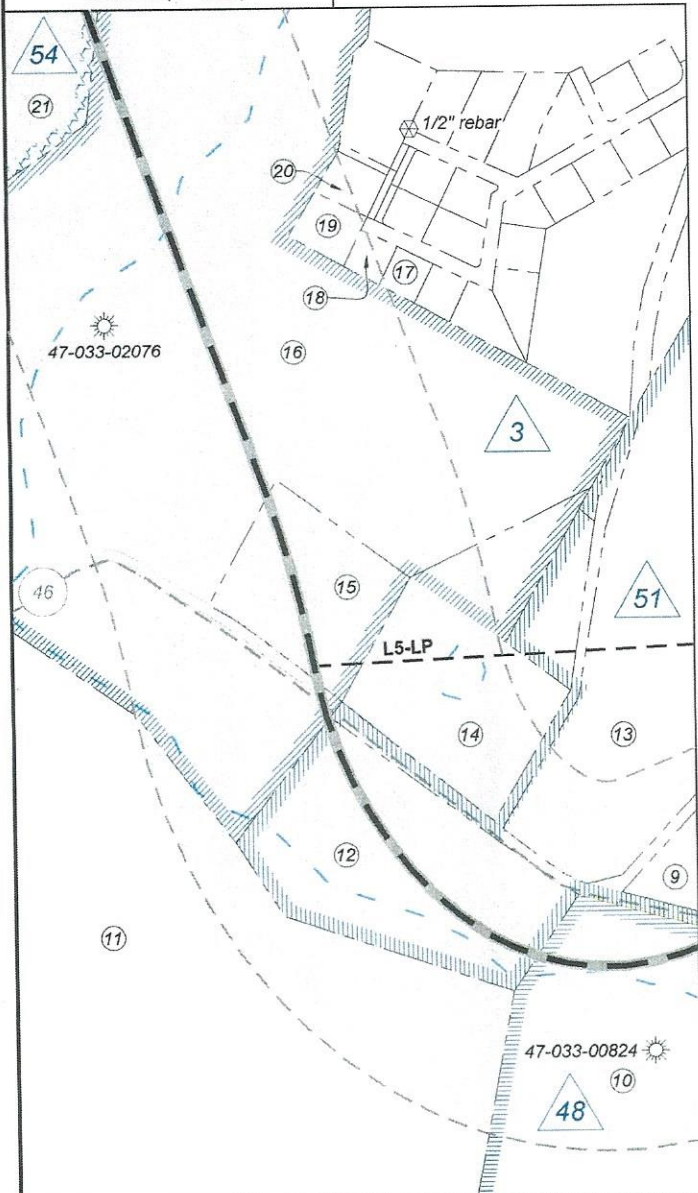
Detail 1 (1"=500')
