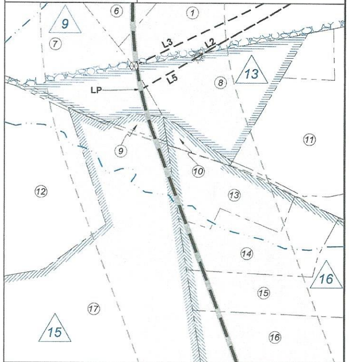
Detail 1 (Scale 1"=500')
