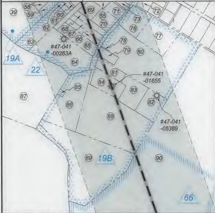
Detail 2 (Scale 1"=500')
