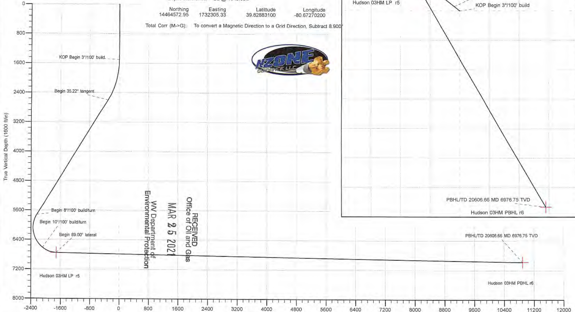
Vertical Section at 156.55° (1600 ft/in)
