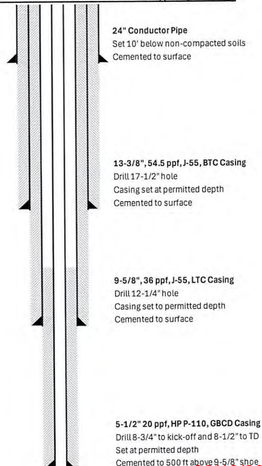
Schematic w/out Mine Contingency String
