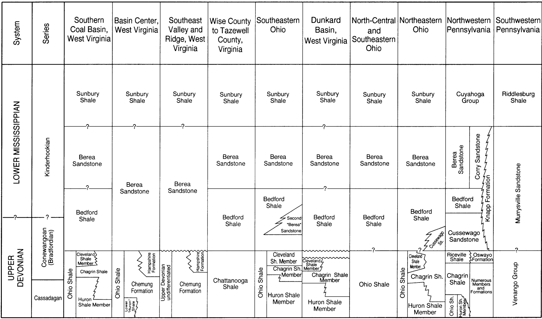
Figure MDe-5. Generalized stratigraphic correlation chart for Upper Devonian through Lower Mississippian strata in the Appalachian basin. Modified from Patchen and others (1985a) and Harper and Laughrey (1989).
