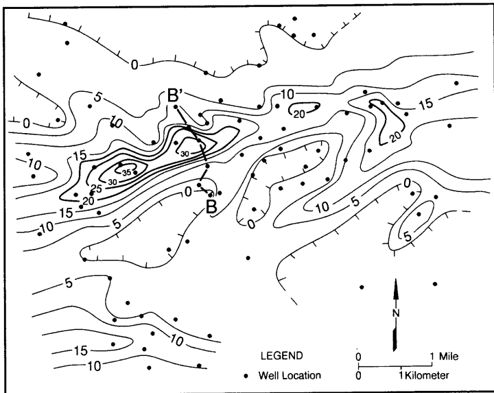
Figure Dbs-24. Sandstone isolith map of an upper Balltown interval (B-3) in the area of the Smicksburg Consolidated field, Indiana County, Pennsylvania. Contour interval = 5 feet. Line of cross section (Figure Dbs-25) is shown. See Figure Dbs-2 for location.
