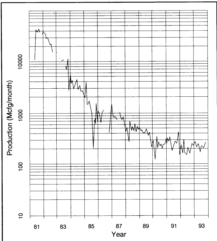
Figure Dbs-29. Typical production decline curve for Kane fractured sandstone (B-1) wells in the Cush Cushion field, eastern Indiana County, Pennsylvania. From Hussing (1994).
