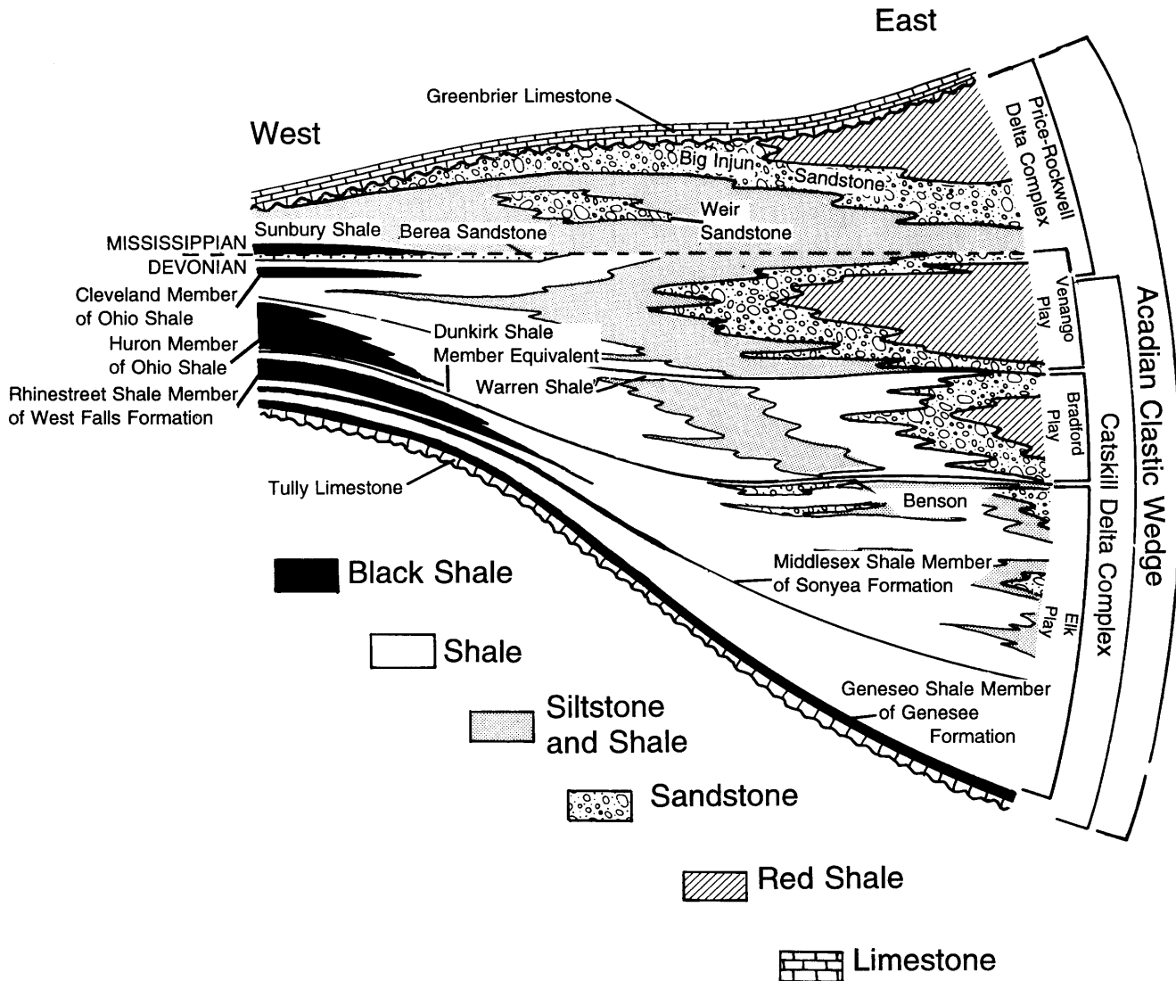
Figure Dbs-3. Diagrammatic cross section of the general lithologic framework of the Acadian clastic wedge showing the relationship of the Price-Rockwell and Catskill delta complexes and the Venango, Bradford, and Elk plays defined in this atlas. The Bradford play represents all the coarse-grained clastic reservoirs occurring between the horizons of maximum regional transgression within the Chadakoin Formation of northern Pennsylvania (equivalent to the informal Warren shale of West Virginia) and the shales just below the Kane sandstone of Pennsylvania (roughly equivalent to the shales immediately overlying the Benson sandstone in northern West Virginia).
