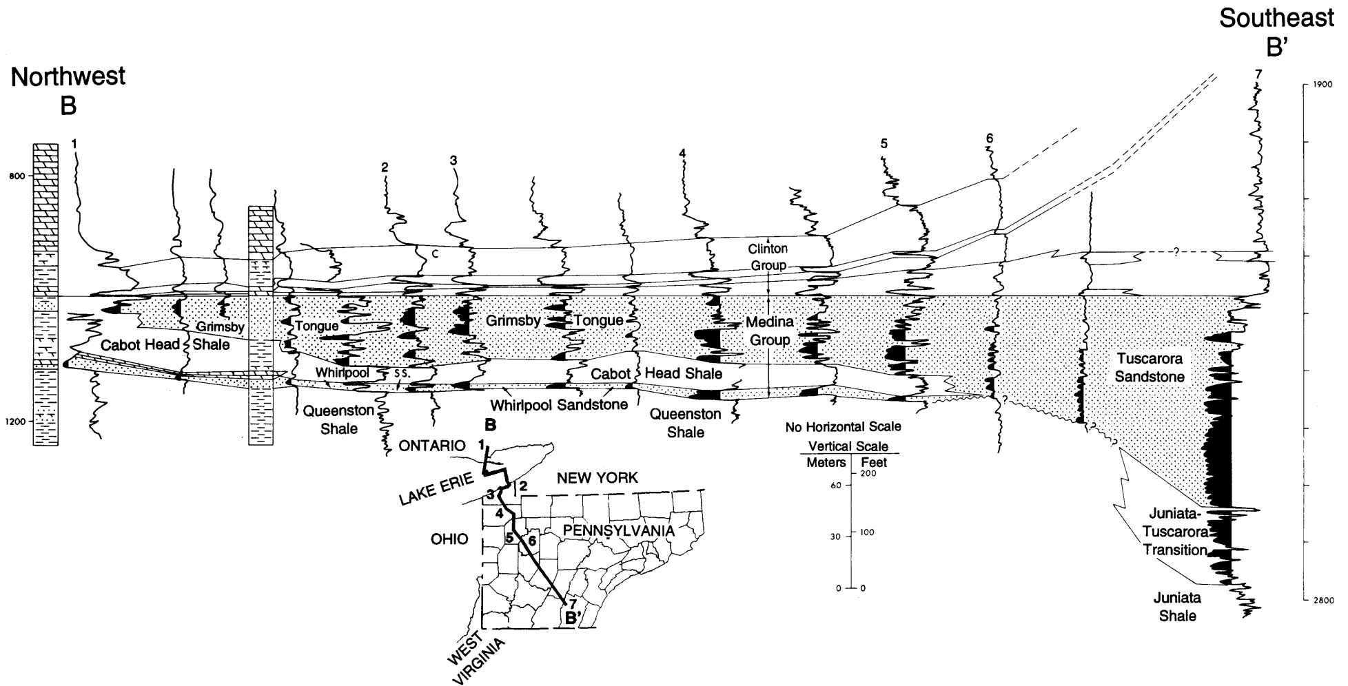
Figure Scm-5. Regional stratigraphic dip cross section B-B' of the Cataract/Medina Group interval. Modified from Piotrowski (1981). Nomenclature is that of Piotrowski (1981).
