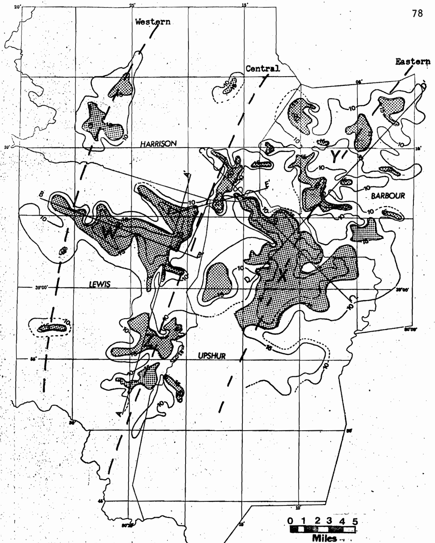
Figure 26. Three arcuate trends (dotted lines) in the upper sand of the Benson zone isolith map. Also shown are sandy areas W, X, Y and Z and cross section locations (solid lines).
