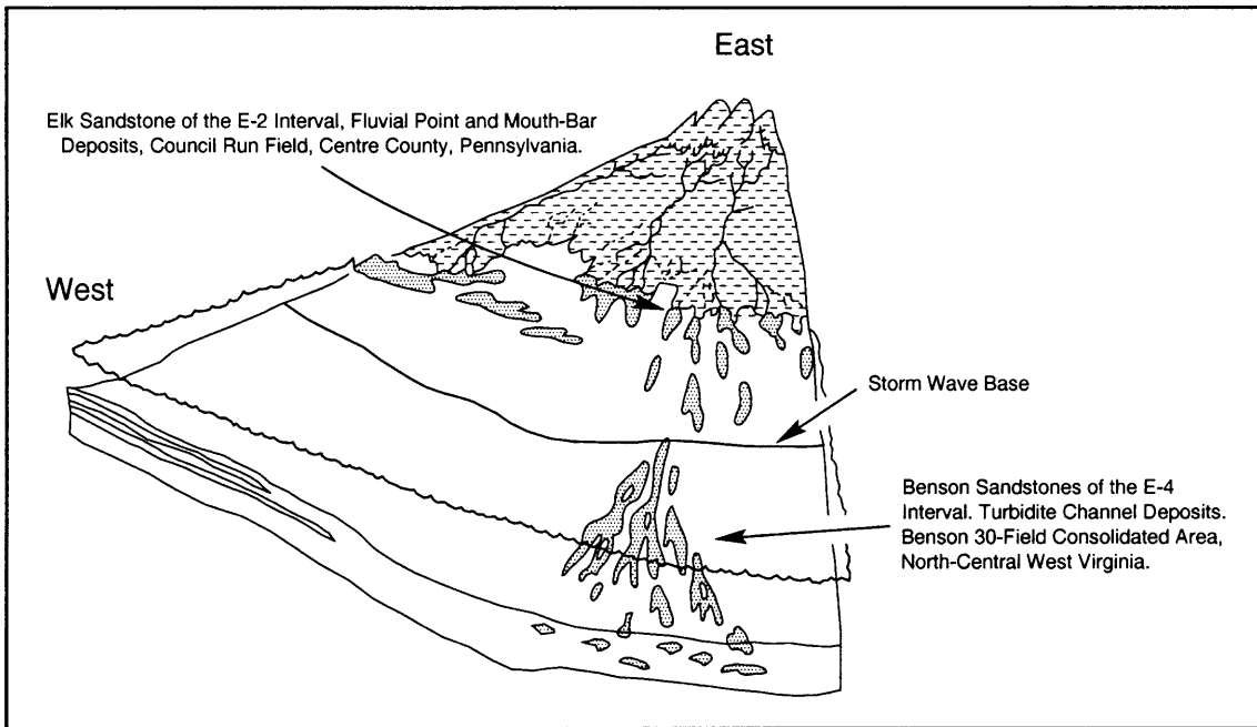
Figure Des-8. Diagram showing the interpreted slope apron depositional setting for the E-4 Benson in the 30-field consolidated area of north-central West Virginia and the shoreline-delta plain setting of the E-2 sandstone in the Council Run field of north-central Pennsylvania.
