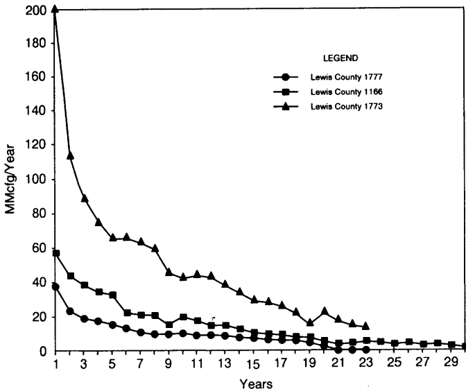
Figure Des-25. Decline curves for three wells in the Weston-Jane Lew field, Lewis County, West Virginia. Locations of wells are shown in Figure Des-24.
