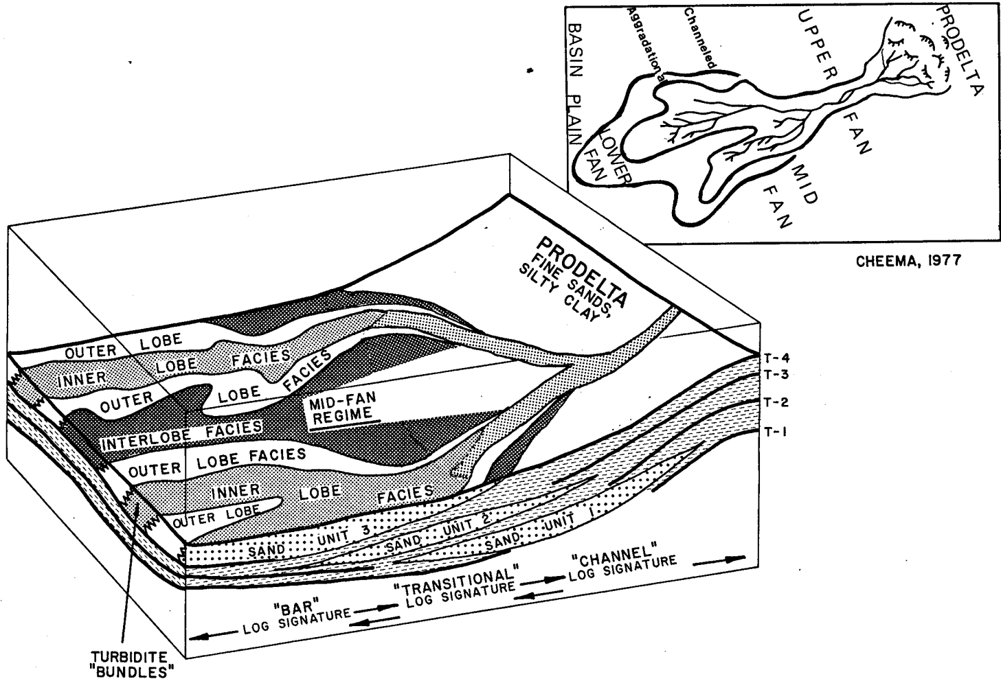
FIGURE 35. SUGGESTED DEPOSITIONAL MODEL FOR BENSON
