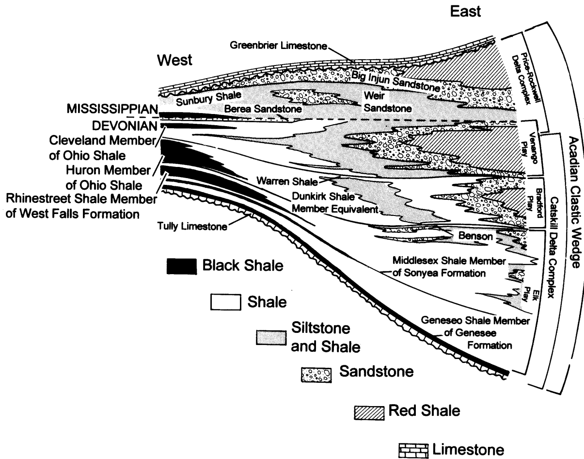
Figure Des-4. Schematic diagram of the Acadian clastic wedge, showing the relationship of the Price-Rockwell and Catskill delta complexes, three Upper Devonian sandstone and siltstone plays with their key bounding units noted, and the general lithologic framework. The Elk sandstone and siltstone play is the basal part of the Catskill delta complex.
