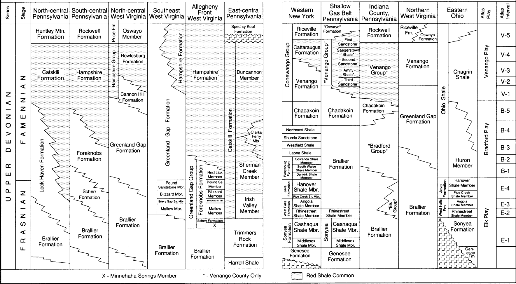
Figure Des-5. Regional correlation chart of the Upper Devonian Catskill delta complex. Modified from Boswell and others (1987) and Woodrow and others (1988).
