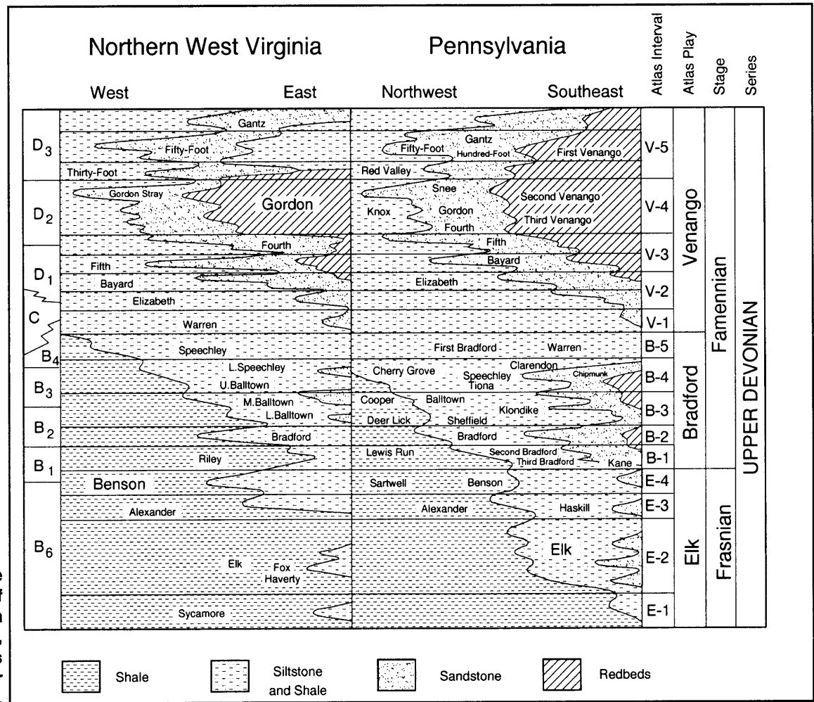
Figure Des-6. Generalized stratigraphic section showing the sequence and approximate correlation of major drillers' units in the subsurface of western Pennsylvania and northern West Virginia. Pennsylvania correlations taken largely after Fettke (1938b), Dickey and others (1943), Wolfe (1963), and Harper and Laughrey (1987). West Virginia correlations after Cardwell (1982a), Filer (1985), and Boswell and others (1987). Far left column shows terminology introduced by Kelley and Wagner (1970).
