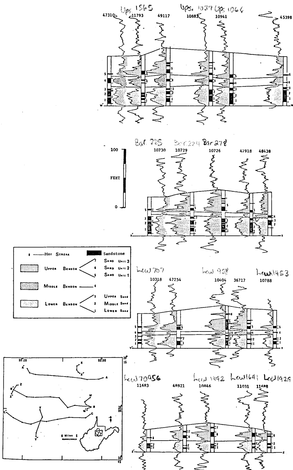
Fig. 8: Transverse (north-south) cross-sections showing gamma-ray log signatures, and geometry of various sandstone units of the Benson interval.
