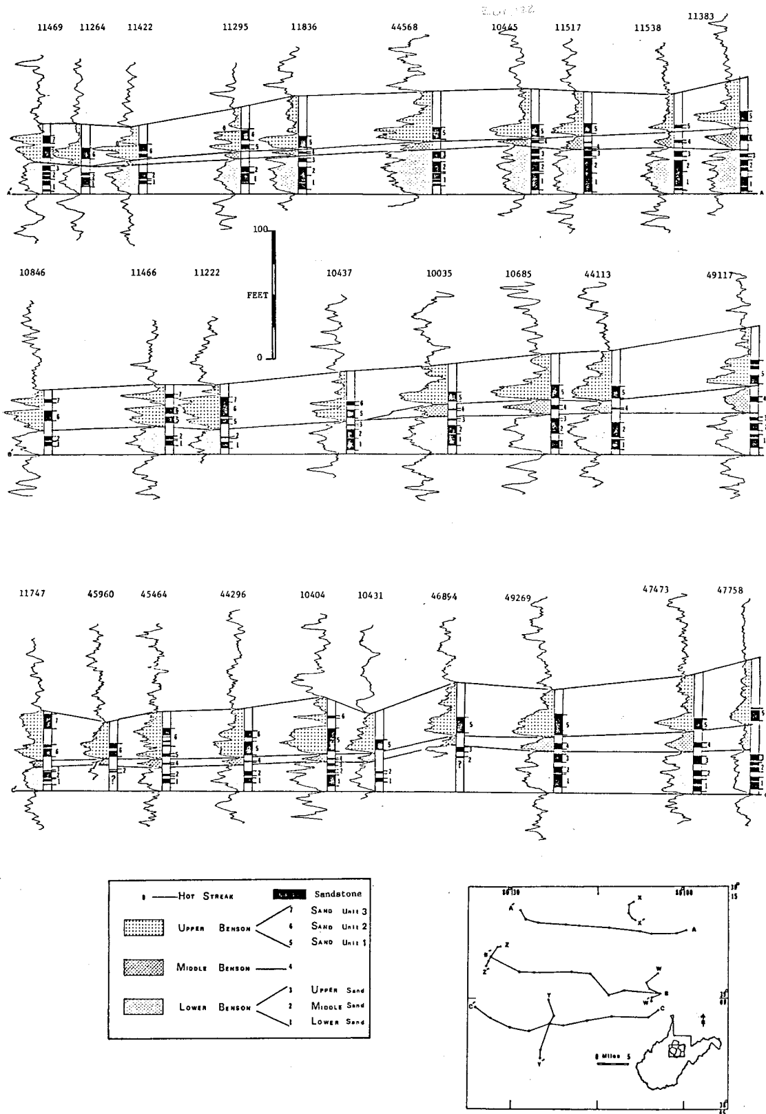
Fig. 7: Longitudinal (east-west) cross-sections showing gamma-ray log signatures, and geometry of various sandstone units of the Benson interval.
