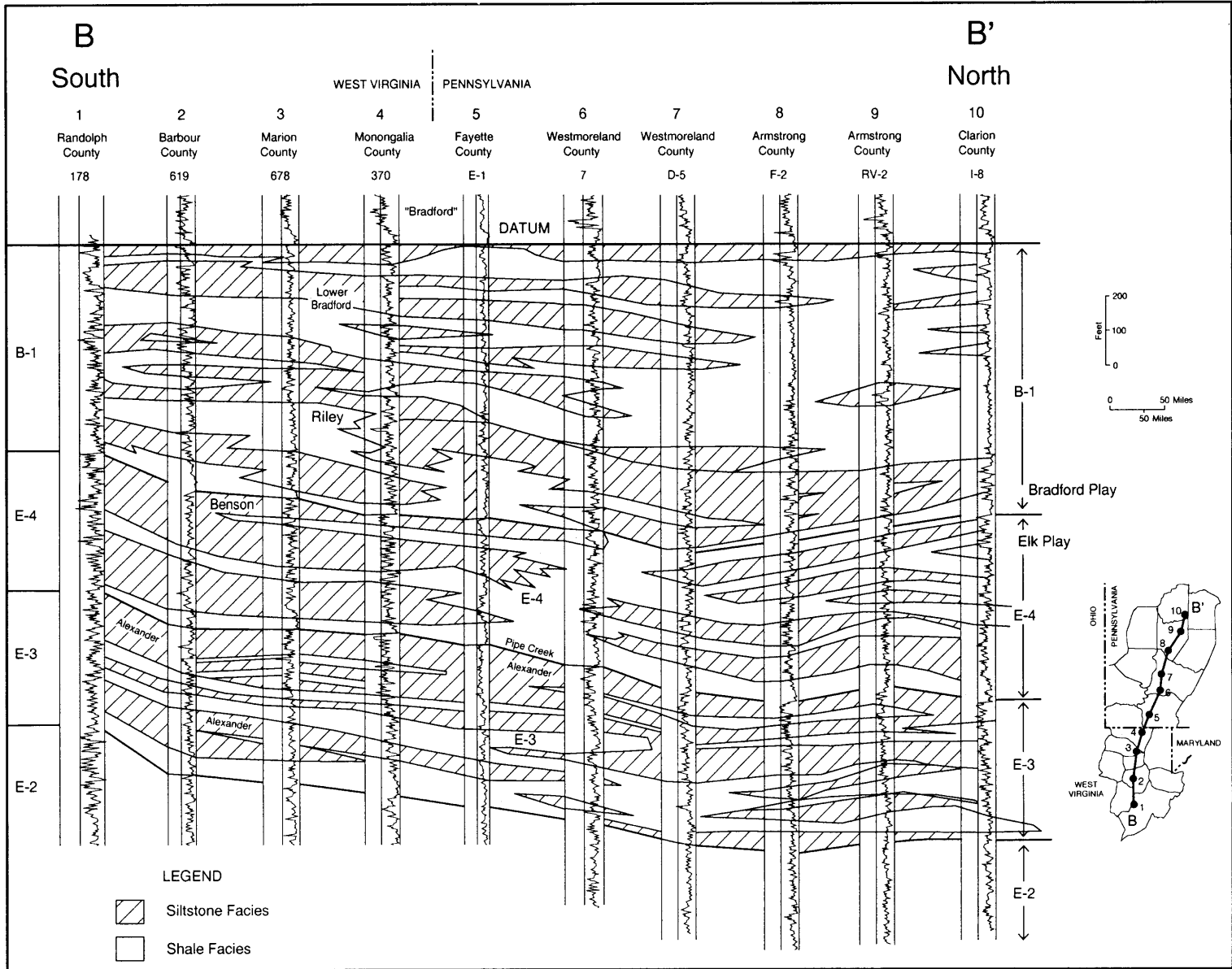
Figure Des-11. Regional gamma-ray stratigraphic cross section of the upper units of the Elk play from northern West Virginia to west-central Pennsylvania. See Figure Des-2 for regional location.
