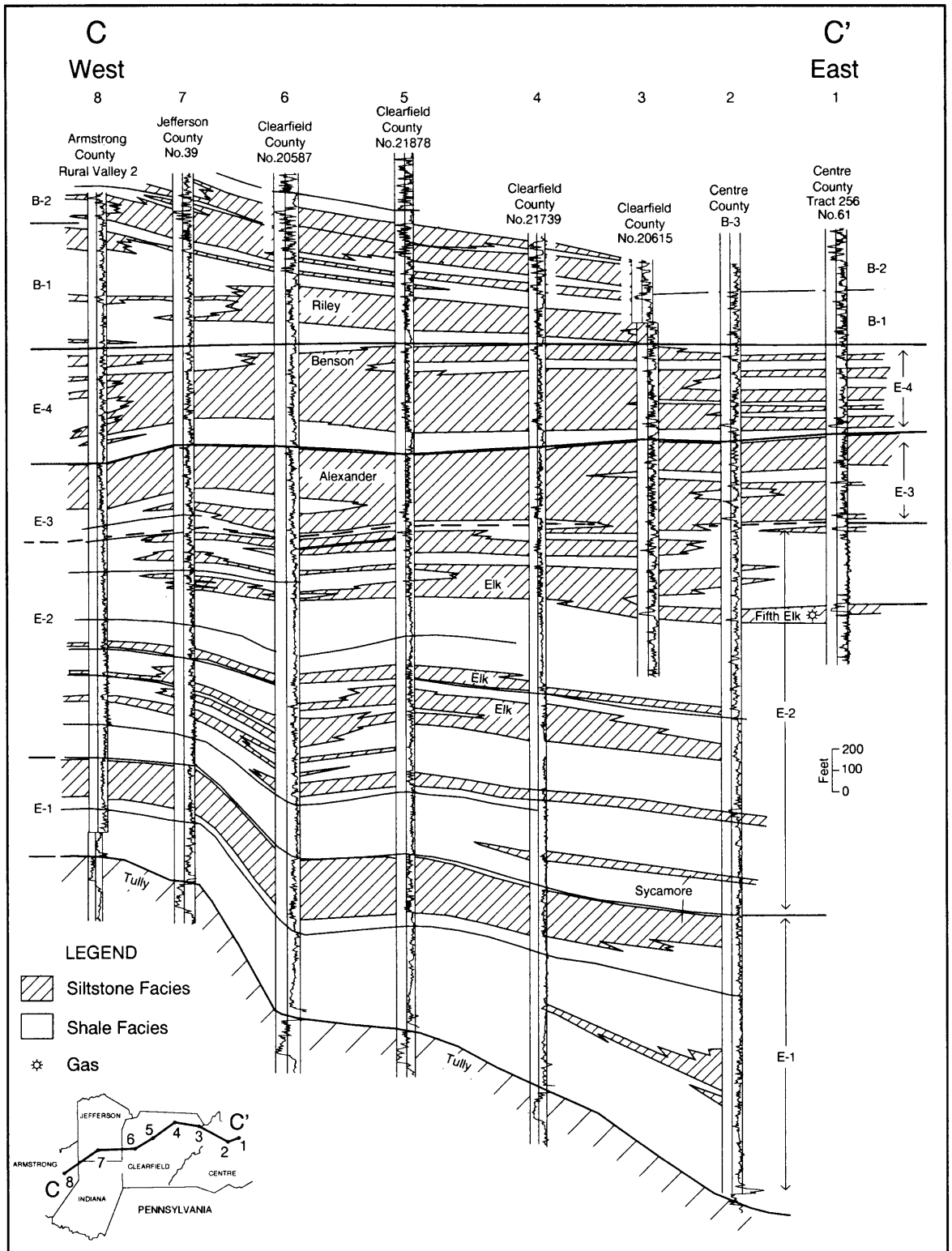
Figure Des-12. Regional gamma-ray stratigraphic cross-section of the Elk sandstone and siltstone in western Pennsylvania. The sequence thins rapidly from east to west. The primary productive reservoir, the Fifth Elk of the Council Run field in Centre and Clinton counties, Pennsylvania, occurs within the E-2 interval. See Figure Des-2 for regional location.
