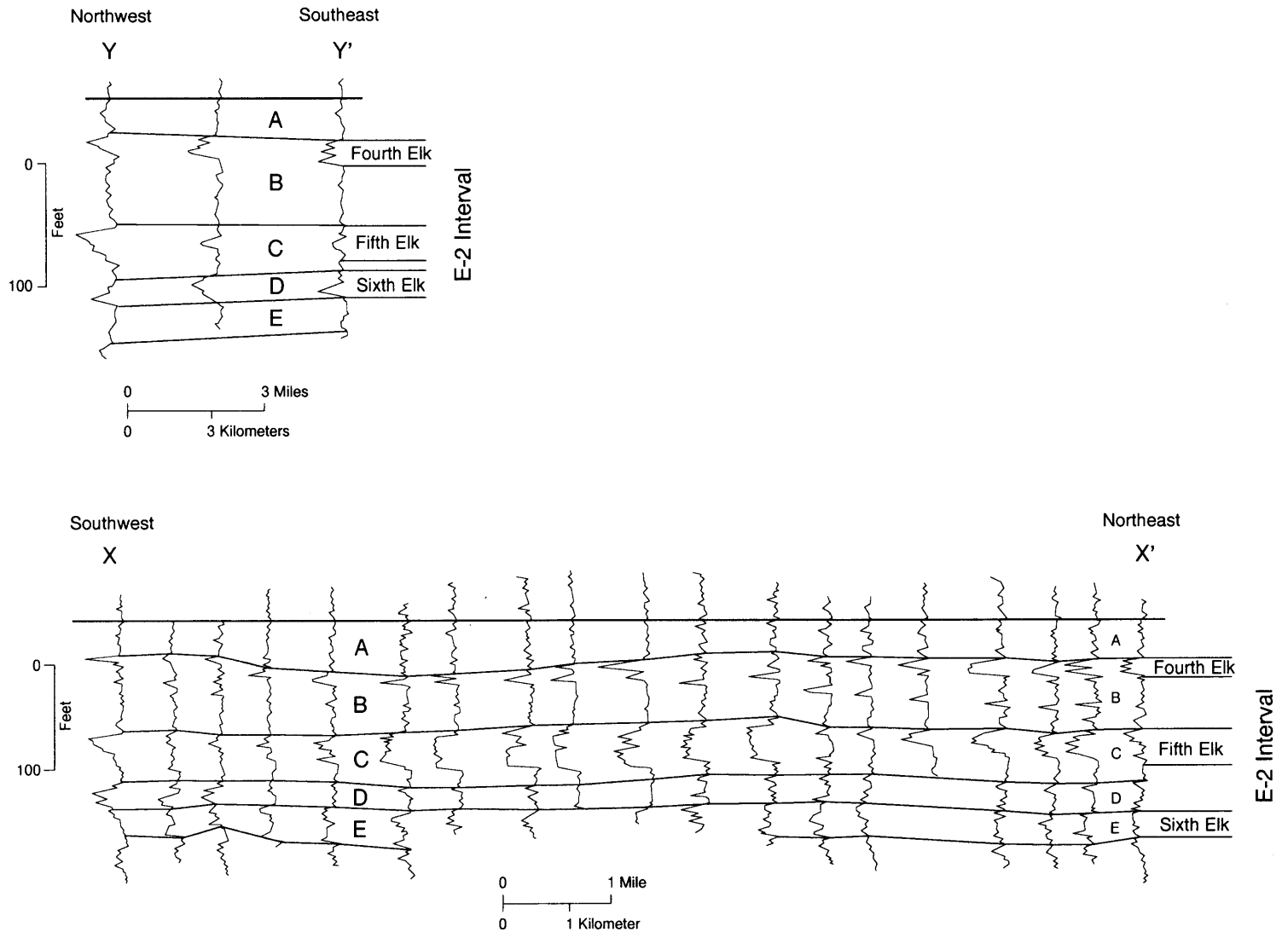
Figure Des-33. Regional gamma-ray log cross sections X-X' (strike trend) and Y-Y' (dip trend) across the Council Run field. The Fifth Elk is the main reservoir. See Figure Des-31 for location of cross sections.
