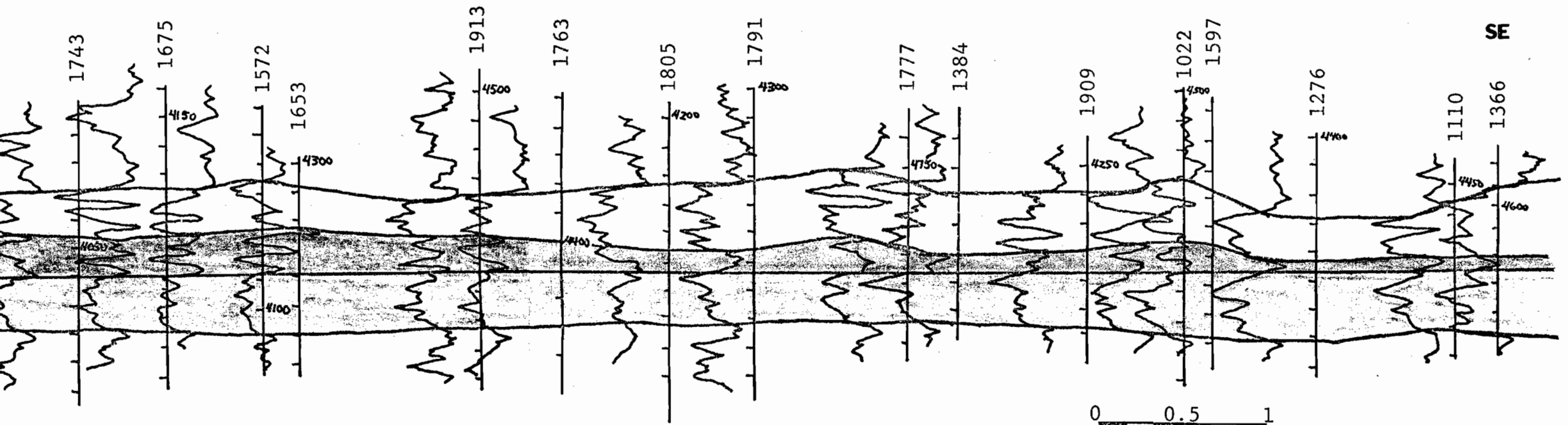
Section B-B' showing the gamma-ray logs for three units of the Benson zone: upper sand, middle shaly interval, and lower sand. Depths on logs are in feet.
