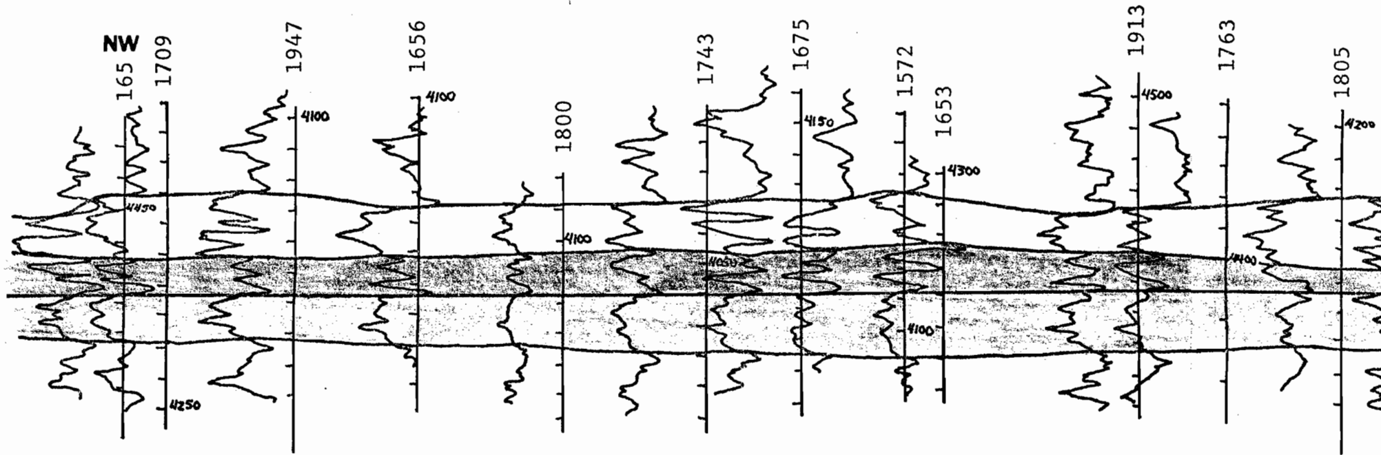
Figure 21. Stratigraphic cross section B-B' showing the gamma-ray log correlation of the three units of the Benson zone based on the bottom of the middle shaly interval as a datum. Numbers listed are well permit numbers. Depths on the vertical scale are drilling depths.
