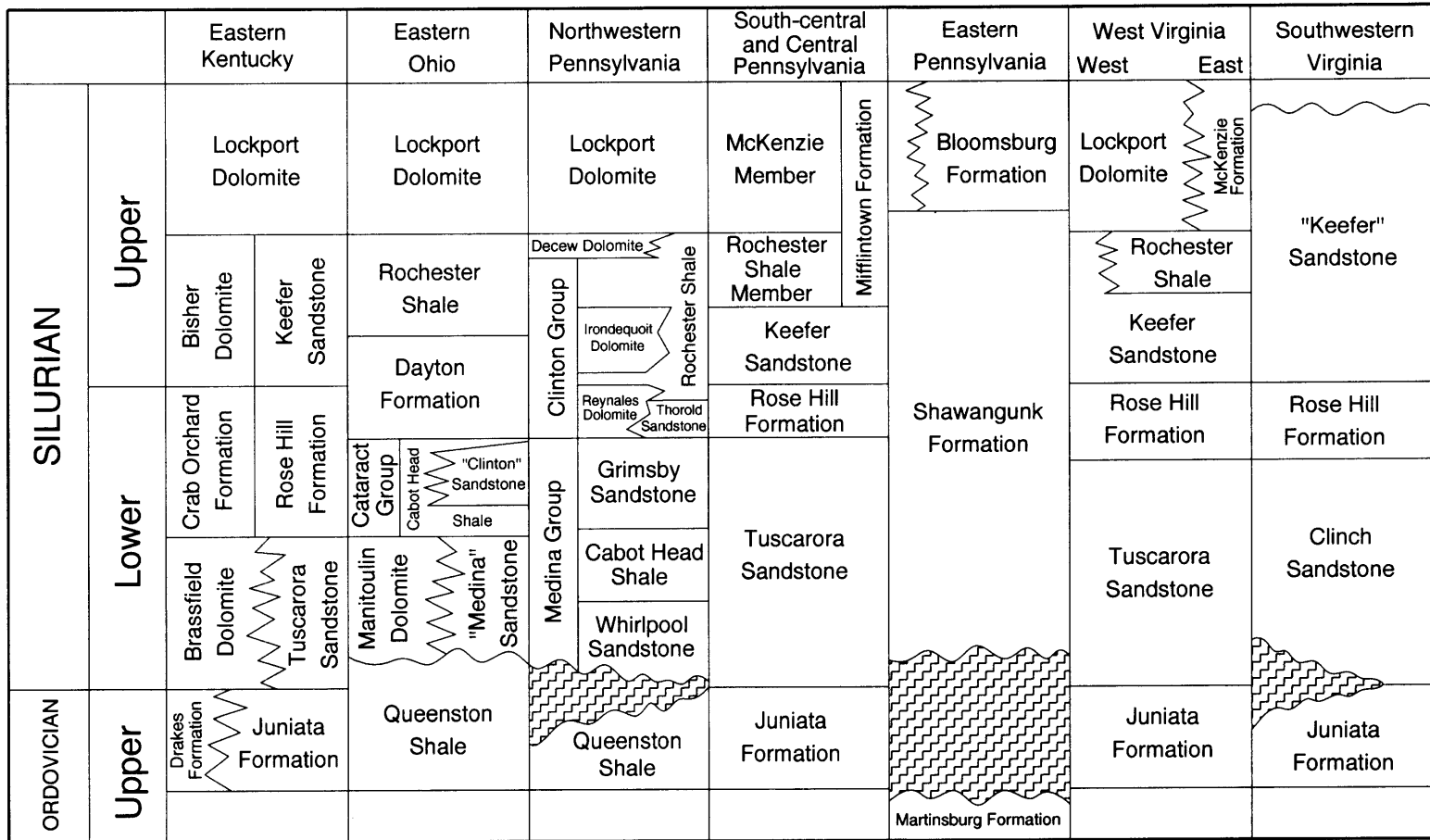
Figure Sts-4. Stratigraphic correlation chart showing the Tuscarora Sandstone and its stratigraphic equivalents. Modified after Patchen and others (1985a). (Avary, 1996)
