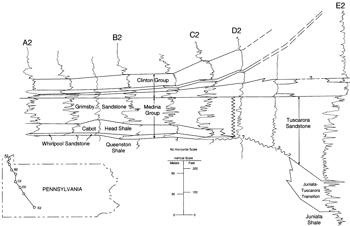
Figure Sts-6. Tuscarora stratigraphic correlations across Pennsylvania. Modified from Piotrowski (1981). This cross section shows an increase in shale content and decrease in thickness from southeast to northwest similar to that shown in Figure Sts-5.
