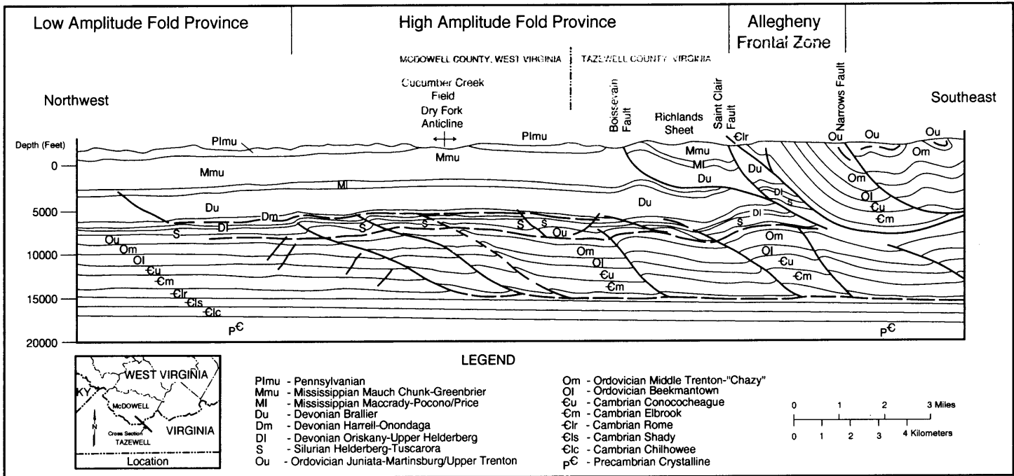
Figure Sts-11. Structural cross section across the Dry Fork anticline modified from Kulander and Dean (1986), illustrating the structural setting and the duplication of the Tuscarora Sandstone by thrust faulting in the Cucumber Creek field, McDowell County, West Virginia. (Avary, 1996)
