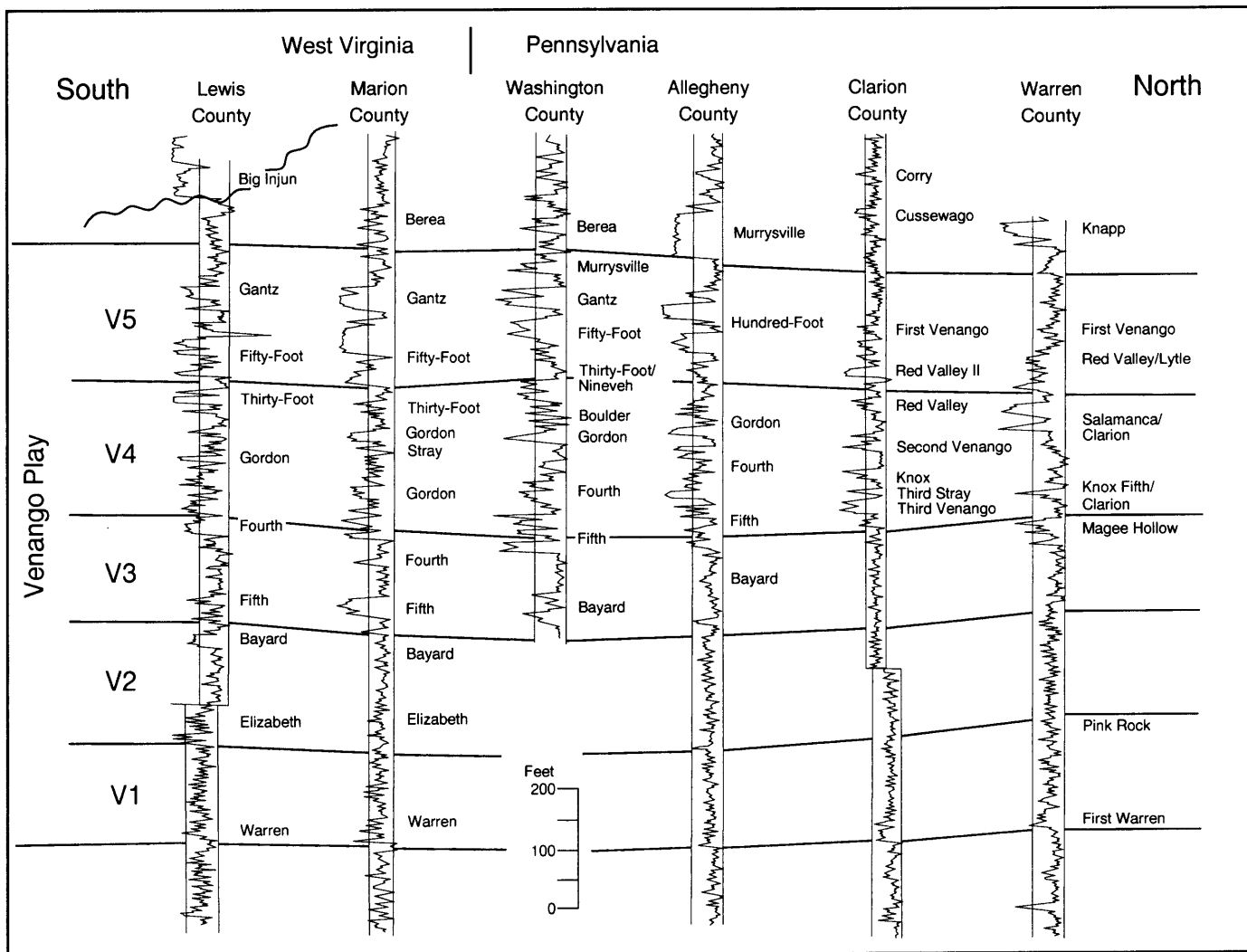
Figure Dvs-7. North-south gamma-ray cross section of the Venango interval from central West Virginia to northwestern Pennsylvania. Designation of intervals V-1 through V-5 are based on regional correlation of Boswell and others (1993). Drillers' names reflect the names most commonly used at that particular horizon in each area. A prominent historical correlation error is the expanded use of the term Gordon in West Virginia, which has resulted in the misnaming of the subadjacent Fifth, Fourth, and Bayard sandstones relative to their original positions in southwestern Pennsylvania. Drillers' names are based on the following: Lewis County, West Virginia, Cardwell (1980); Washington and Allegheny counties, Pennsylvania, McGlade (1967) and Harper and Laughrey (1987); Clarion County, Pennsylvania, Kelley (1967); and Warren County, Pennsylvania, Lytle (1965). No datum or horizontal scale. See locator map for line of cross section.
