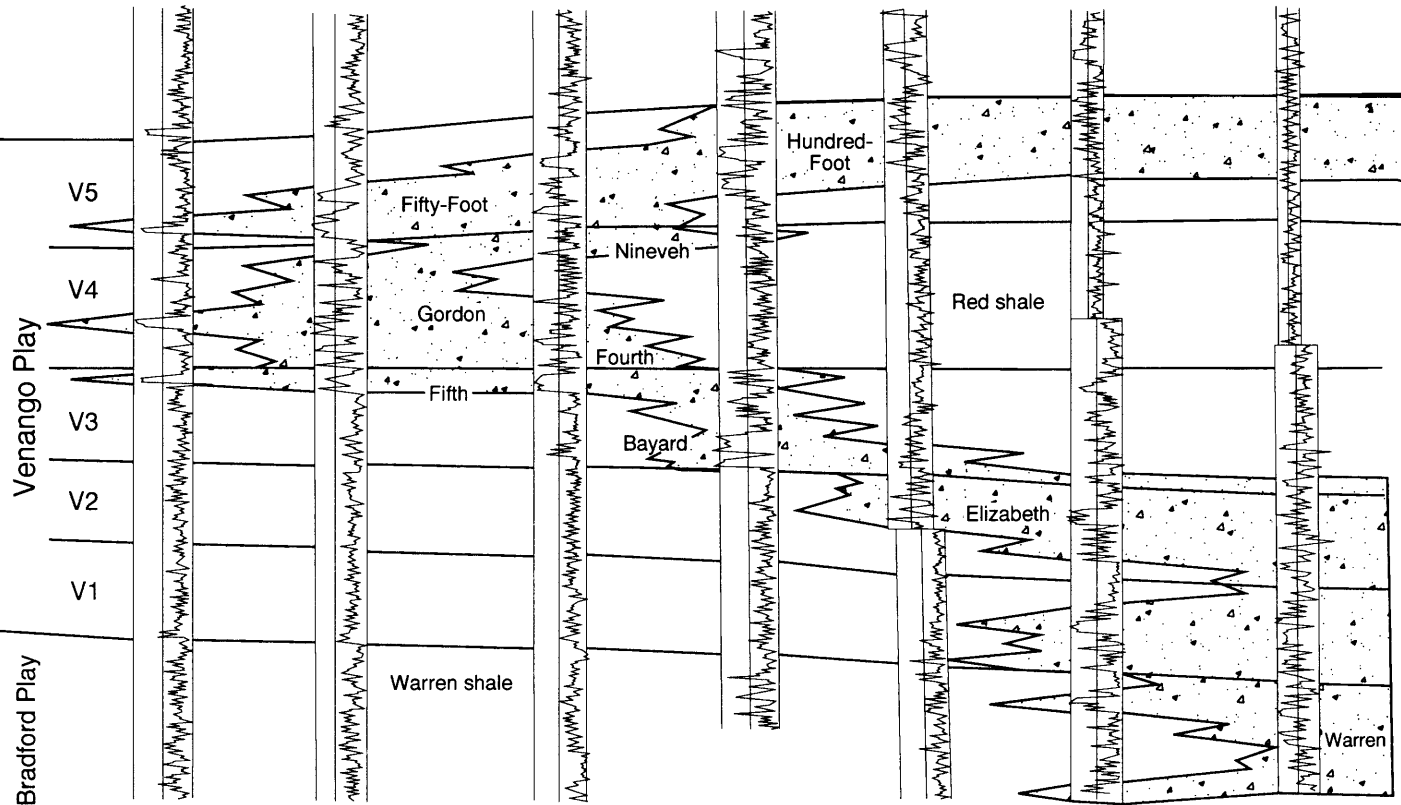
Figure Dvs-8. East-west gamma-ray cross section of the Venango interval in southwestern Pennsylvania. After McGlade (1967) and Harper and Laughrey (1987). Wells are identified by county permit numbers. No datum or horizontal scale. See locator map for line of cross section. (Boswell and others, 1996-Dvs)
