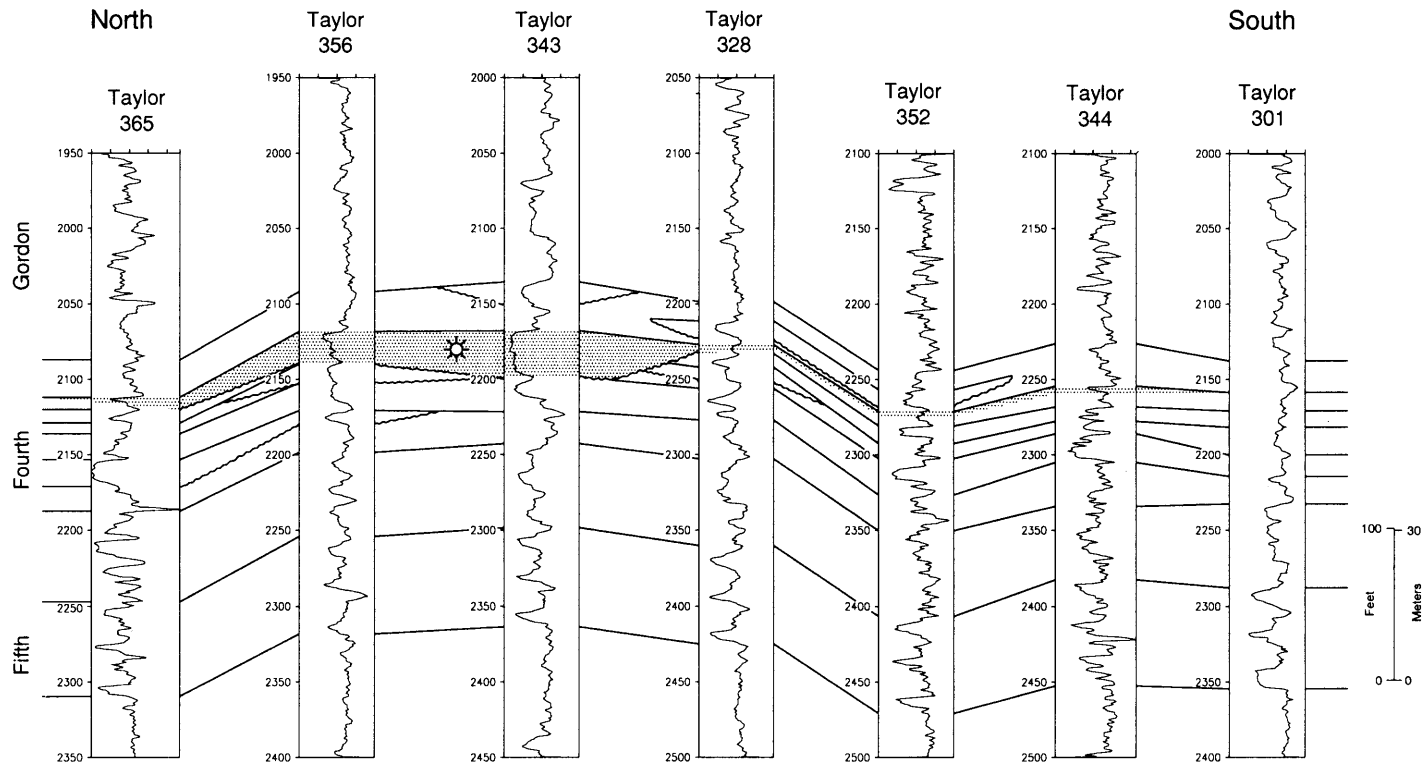
Figure Dvs-19. North-south stratigraphic cross section across area of Venango production, Taylor County, West Virginia. Productive upper part of the Fourth sandstone is indicated by stippling. (Boswell and others, 1996-Dvs)
