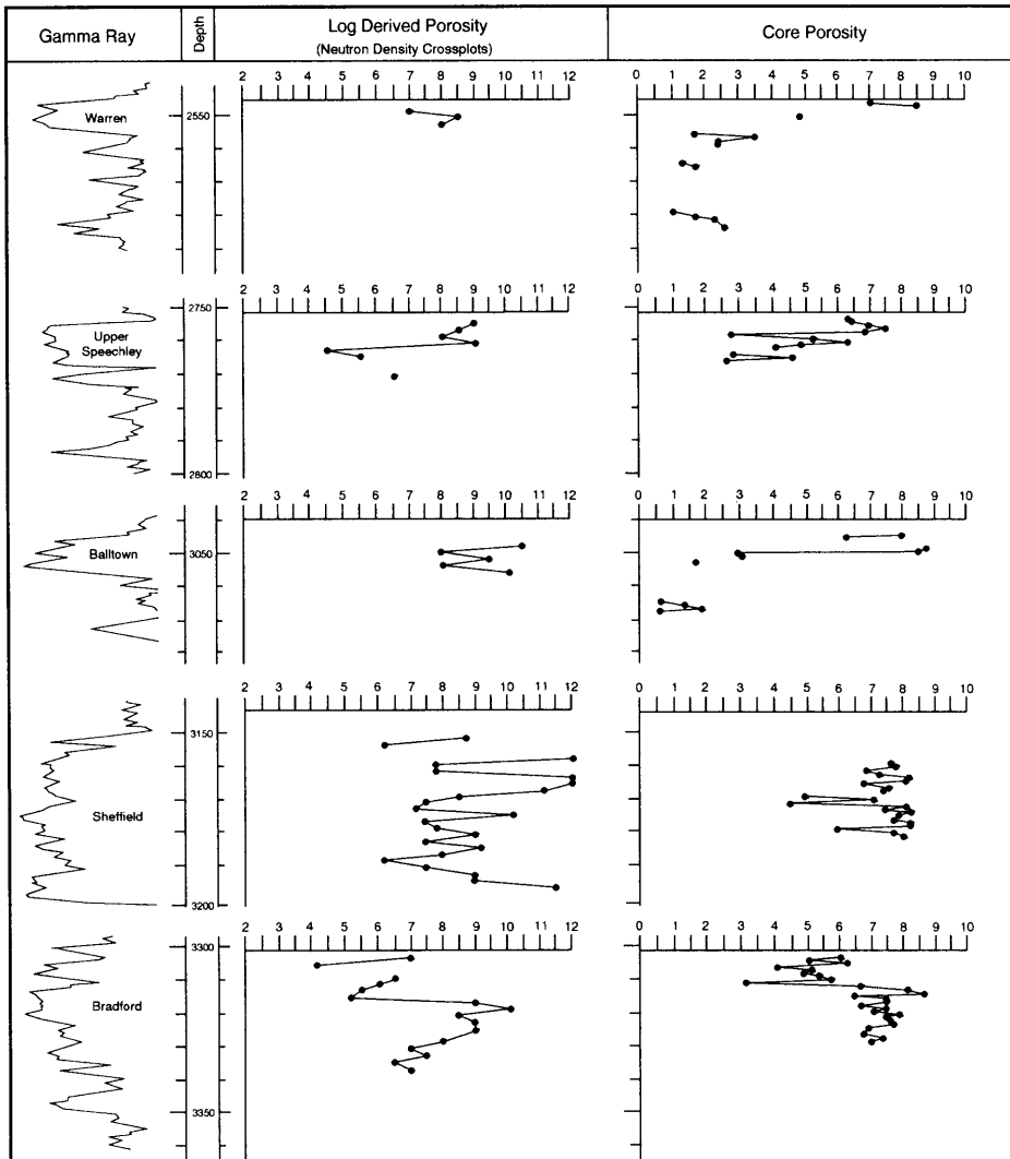
Figure Dbs-18. Comparison of core and log data from various Bradford sandstones in the No. 1 Good, Lahr, and Kaufman well, Indiana County, Pennsylvania. Data taken from Laughrey and Harper (1986). In general, log-derived porosities are greater than core porosities for this well.
