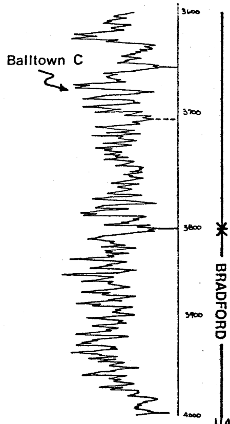
Fig.3 Sample gamma ray log [HAR-BAR-862] of study interval, showing sands and marker shales
