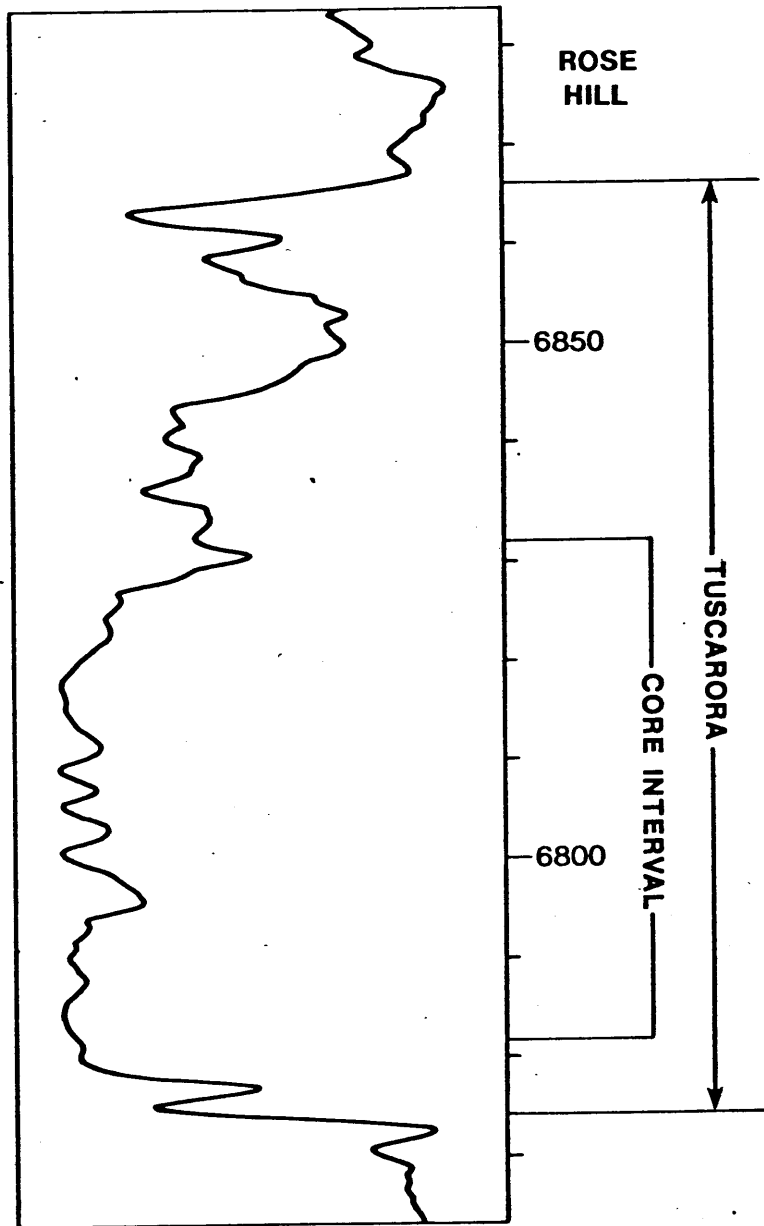
FIG. 5a— Gamma-ray curve of the Tuscarora Sandstone from the David Ward Well #64, Kanawha Co., showing core interval and increasing shaliness toward the top.
