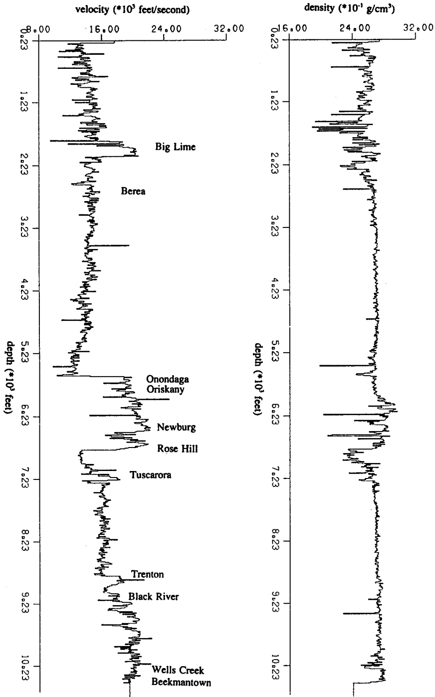
Fig.3.2A Digitized sonic and density log for deep well K3462 in Kanawha County
