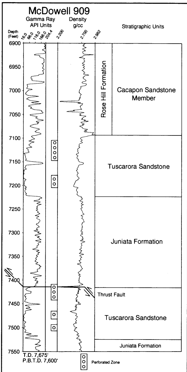
Figure Sts-18. Portion of the gamma-ray and bulk density logs for Conoco Inc. No. 1 Clarence Billups (McDowell 909), Cucumber Creek field discovery well, McDowell County, West Virginia, showing repetition of the Tuscarora Sandstone by thrust faulting.
