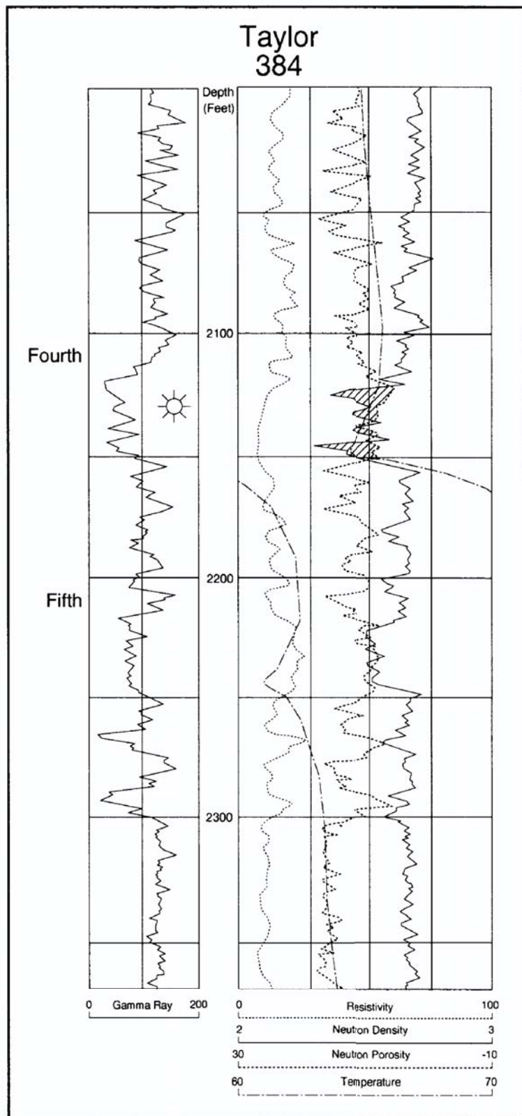
Figure Dvs-22a. Type log of the upper part of the Fourth sandstone, Taylor County, West Virginia. Similar reservoir characteristics have been observed in the Fifth sandstone in east-central Fayette County, Pennsylvania (Figure Dvs-22b).
