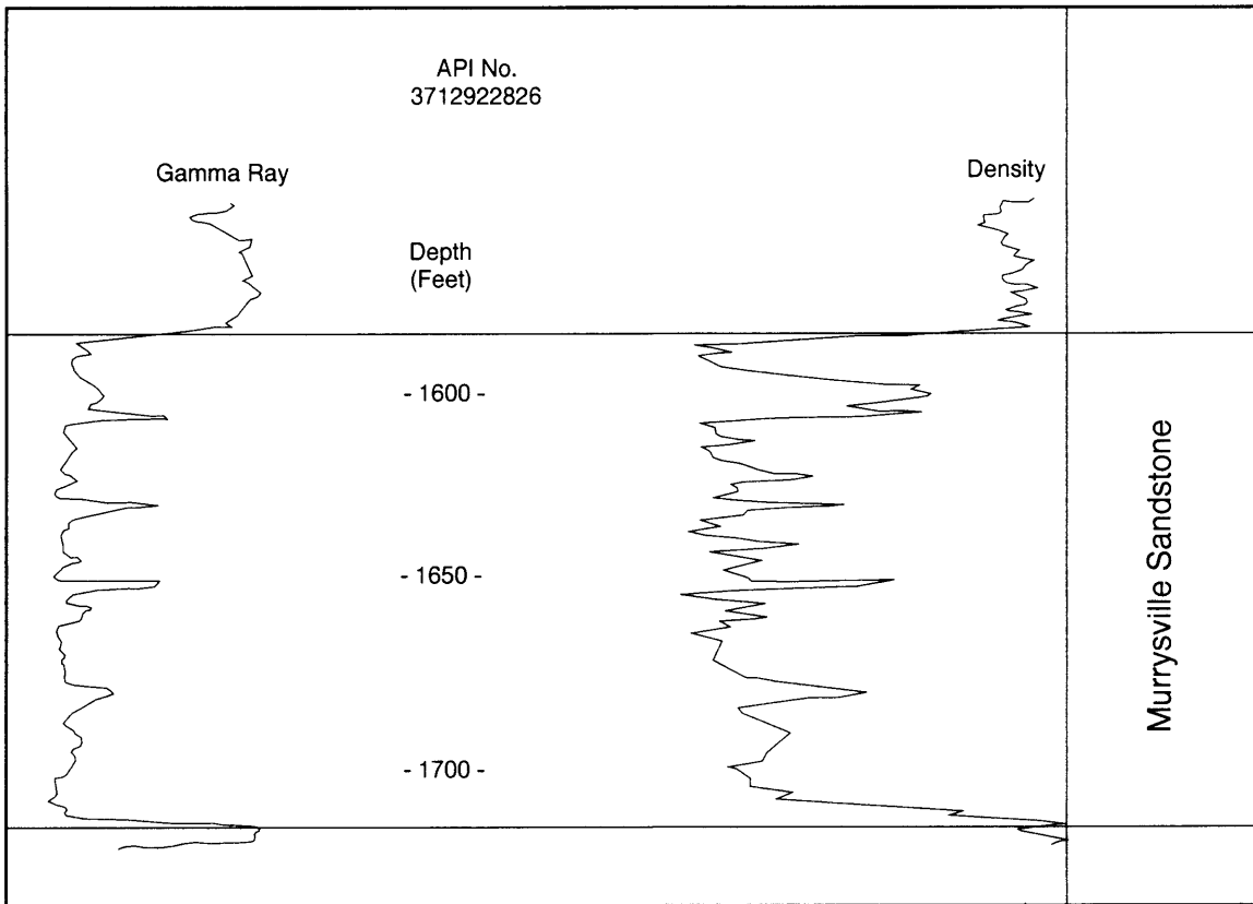
Figure MDe-25. Type geophysical log (API No. 3712922826) for the Murrysville sandstone in the Oakford field, Westmoreland County, Pennsylvania.
