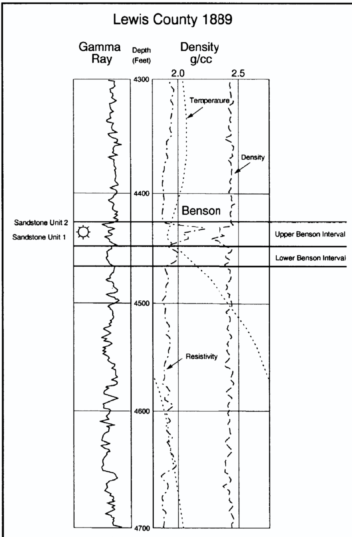
Figure Des-23a. Type log of the Benson E-4 interval in the Weston-Jane Lew field, Lewis County, West Virginia. See Figures Des-22 and Des-24 for location.
